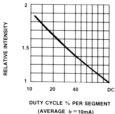
Fig.5 LUMINOUS INTENSITY VS. DUTY CYCLE (AVERAGE I_F = 10\text{mA} )
