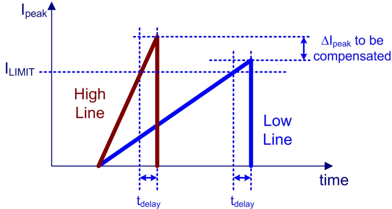
Figure 66. Needs for Line Compensation For True Overpower Protection
