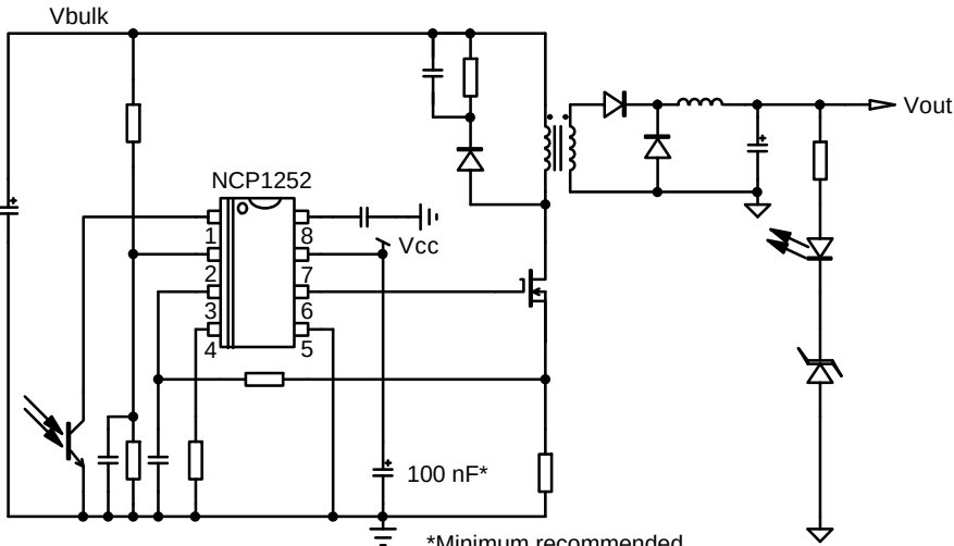
Figure 1. Typical Application
