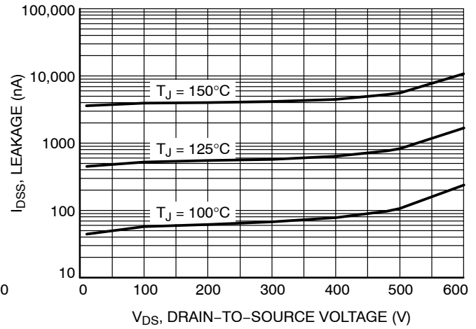
Figure 8. Drain-to-Source Leakage Current vs. Voltage
