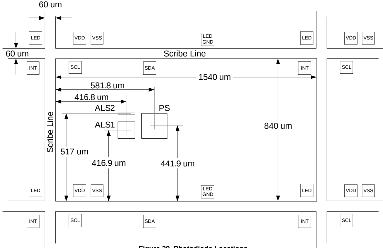
Figure 29. Photodiode Locations
