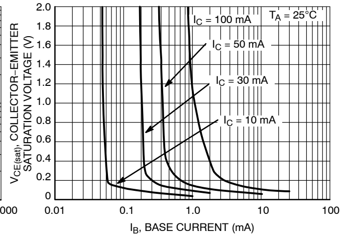
Figure 4. Saturation Region
