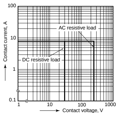
1.-(2) Maximum switching power (1 Form A 1 Form B, 2 Form A)
