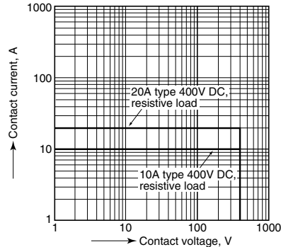
3.-(2) Switching life and cut-off curves (20A type)
