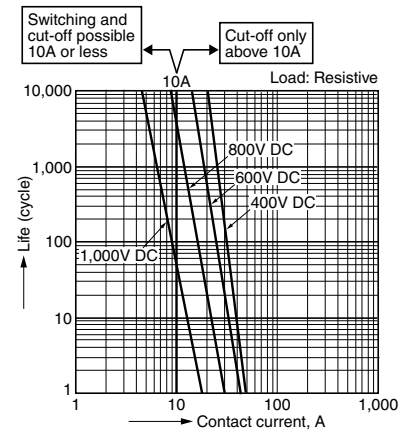
3.-(1) Switching life and cut-off curves (10A type)
