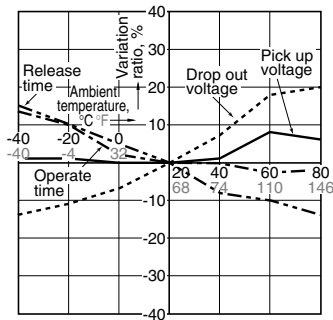
1.-(5) Ambient temperature characteristics (300A type) Tested sample: AEP19012, 3pcs
