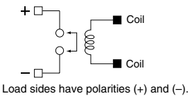
Schematic (Top view)
