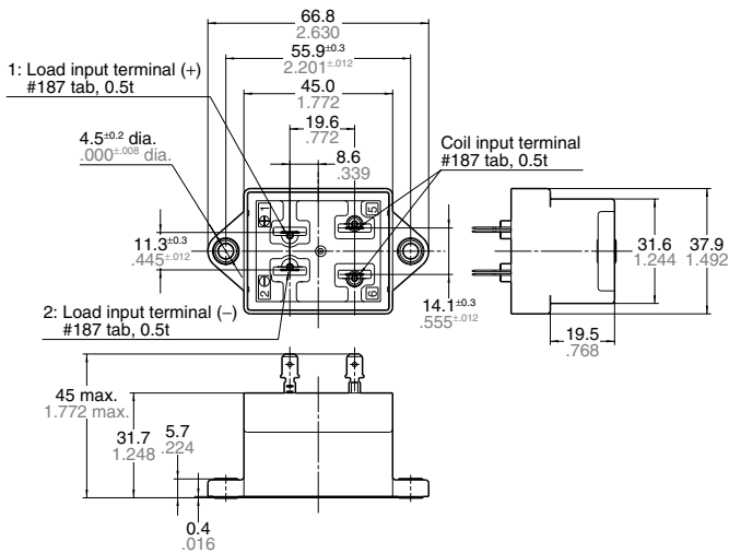
External dimensions
