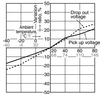
1.-(4) Ambient temperature characteristics (200A type) Tested sample: AEP17012, 3pcs
