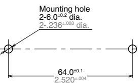
Panel cut-off
