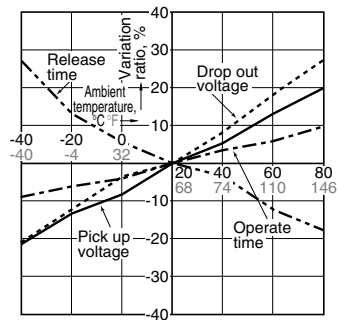
1.-(3) Ambient temperature characteristics (80A type) Tested sample: AEP18012, 3pcs
