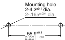
Panel cut-off
