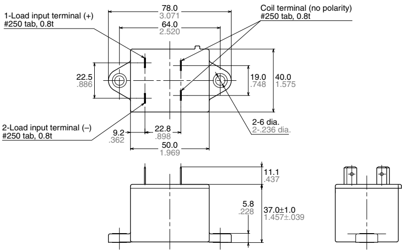
External dimensions
