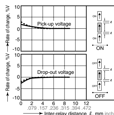
9-(2). Influence of adjacent mounting Tested sample: AGN20012, 6 pcs.
