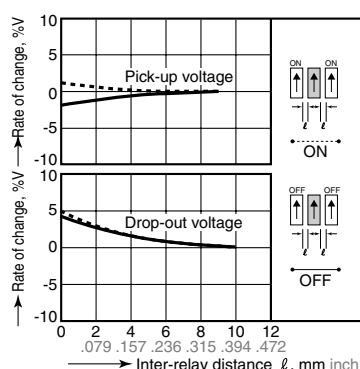
9-(1). Influence of adjacent mounting Tested sample: AGN20012, 6 pcs.
