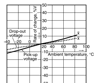
7. Ambient temperature characteristics Tested sample: AGN2004H, 6 pcs.
