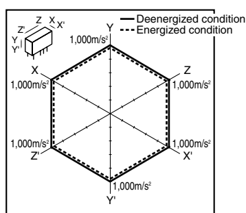
8. Malfunctional shock Tested sample: AGN2004H
