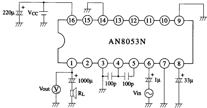
Test Circuit 8
