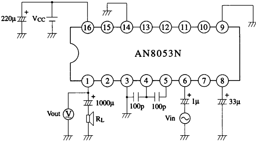
Test Circuit 6
