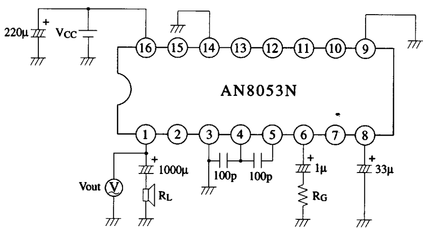
Test Circuit 8
