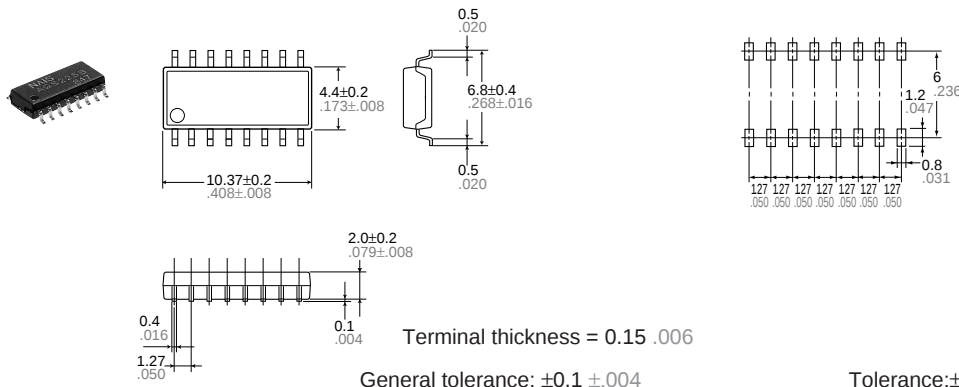
Recommended mounting pad (Top view)
