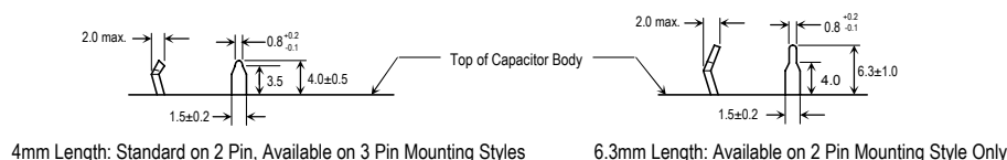
Pin Dimensions
