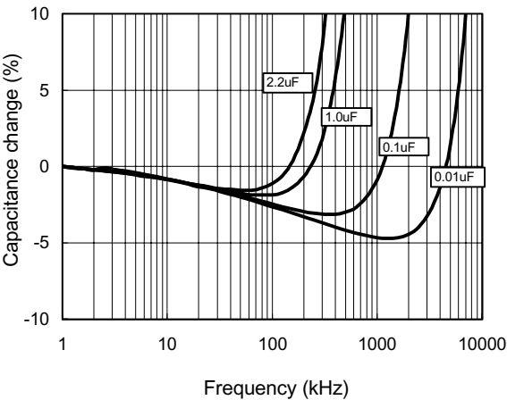
Frequency Characteristics
