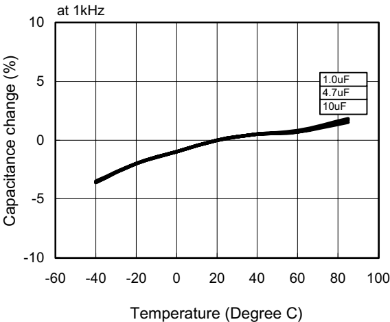
Temperature Characteristics
