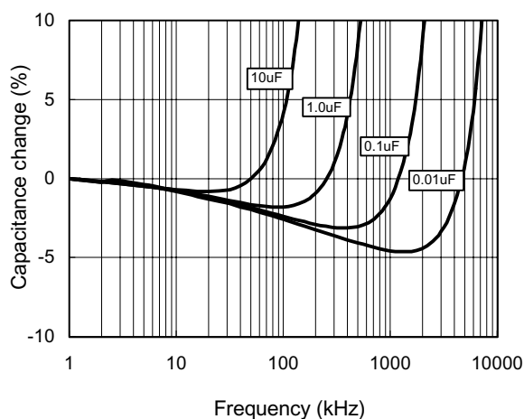
Frequency Characteristics
