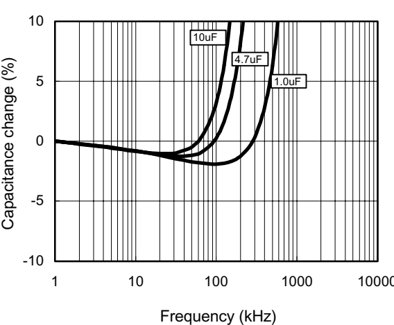
Frequency Characteristics
