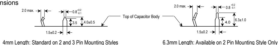
Pin Dimensions
