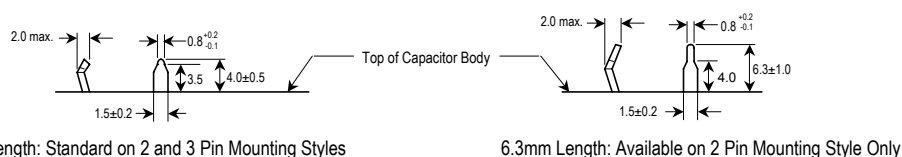
Pin Dimensions
