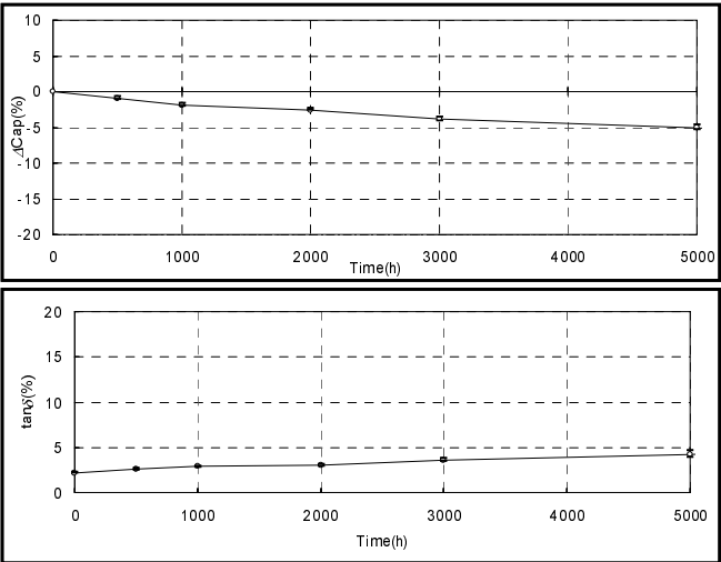
EEVEB2E470 (250V47 \mu F, \phi 16x21.5L)
