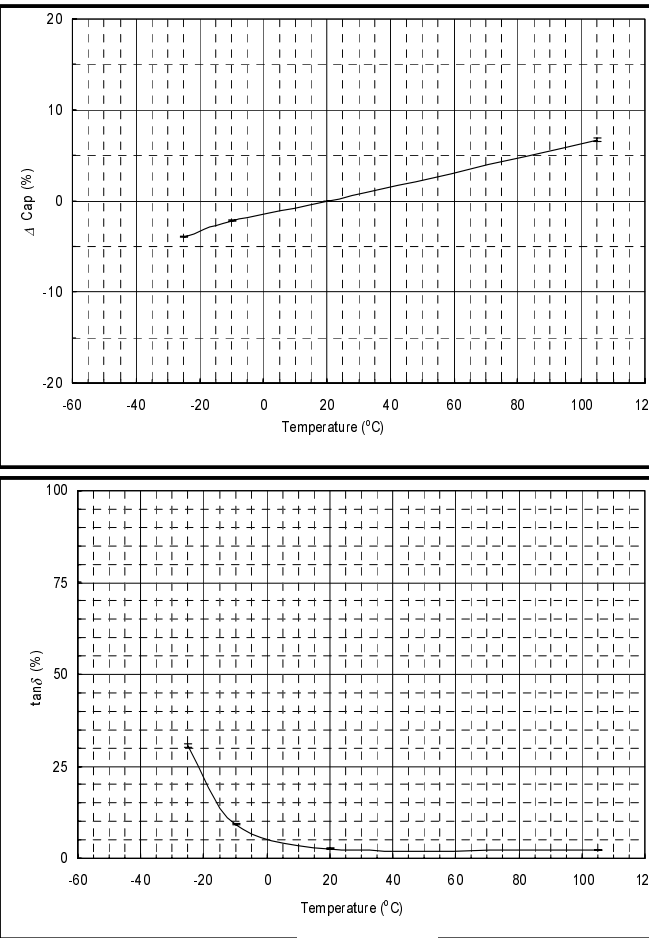
EEVEB2E470 (250V47 \mu F, \phi 16x21.5L)
