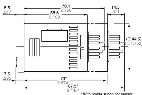
Pin type (Flush mount/Surface mount)
