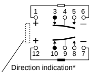
Schematic (Bottom view) 2 coil latching (Reset condition)
