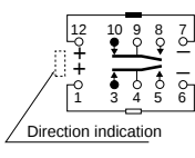
Schematic (Top view) 1 coil latching (Reset condition)
