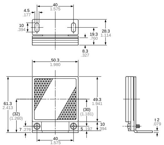
Mounting drawing
