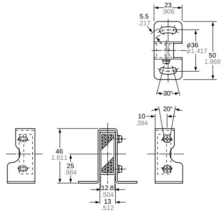
Mounting drawing
