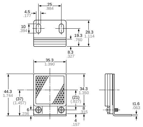
Mounting drawing
