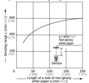
Object size – Sensing range correlation
