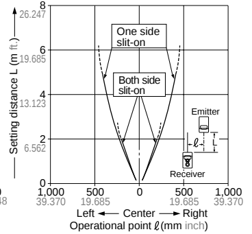
Parallel deviation with rectangular slit masks ( 2 \times 6\text{mm} .079 \times .236inch)
