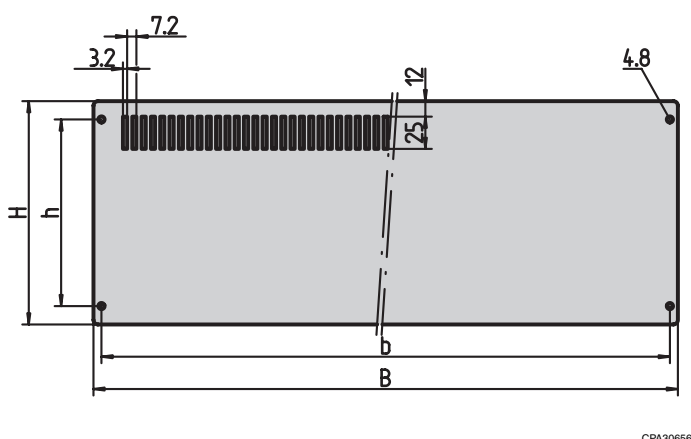
Rear panel/front panel
