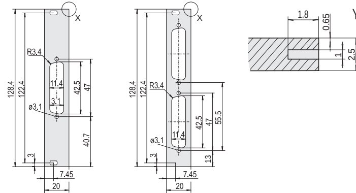
Cut-out 25-pin
