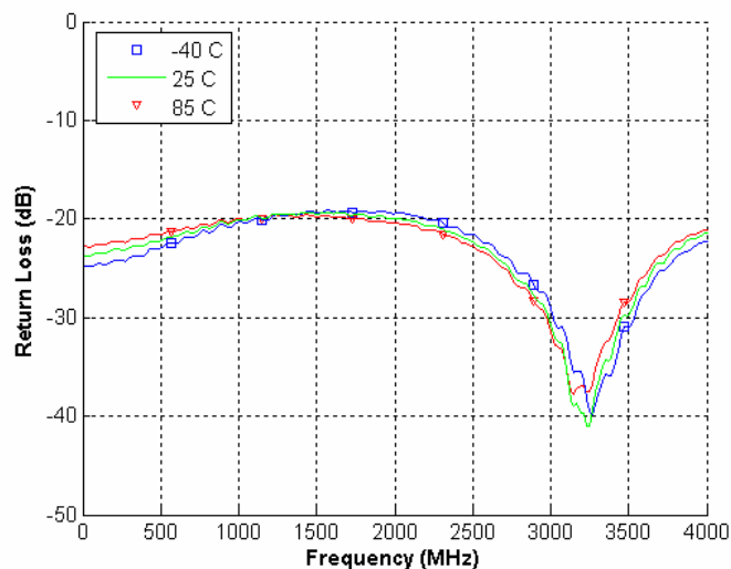
Figure 18. Return Loss: RFC-RF2 @ 3 V
