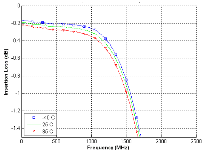
Figure 10. Tx Insertion Loss, V_{DD}=3.3V
