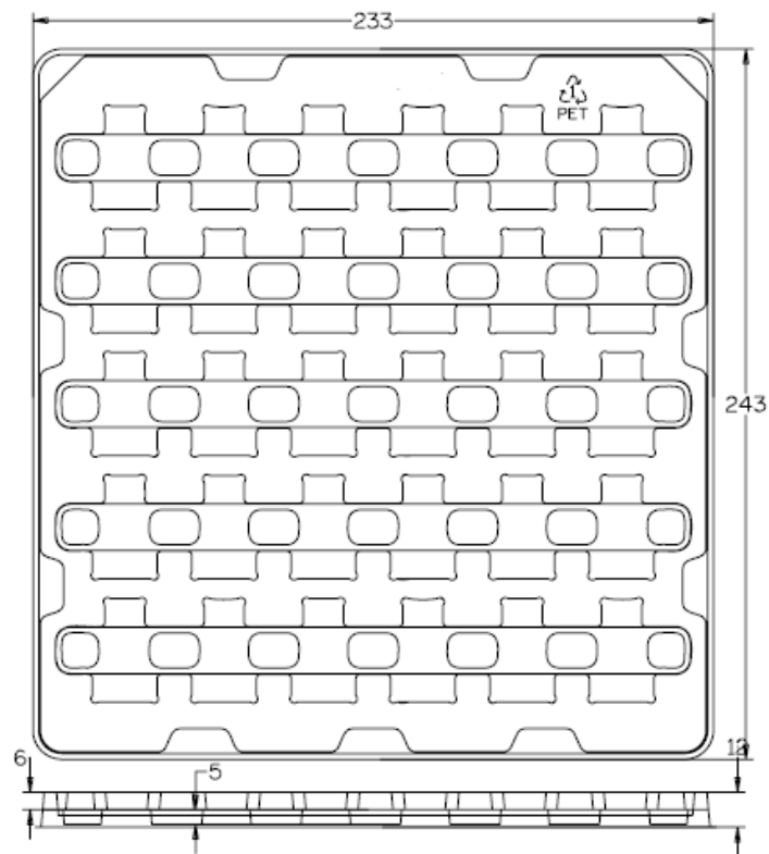
Figure 21. Package ray dimensions for LUXEON S5000 LXSx-Pxxx-004I(N).
