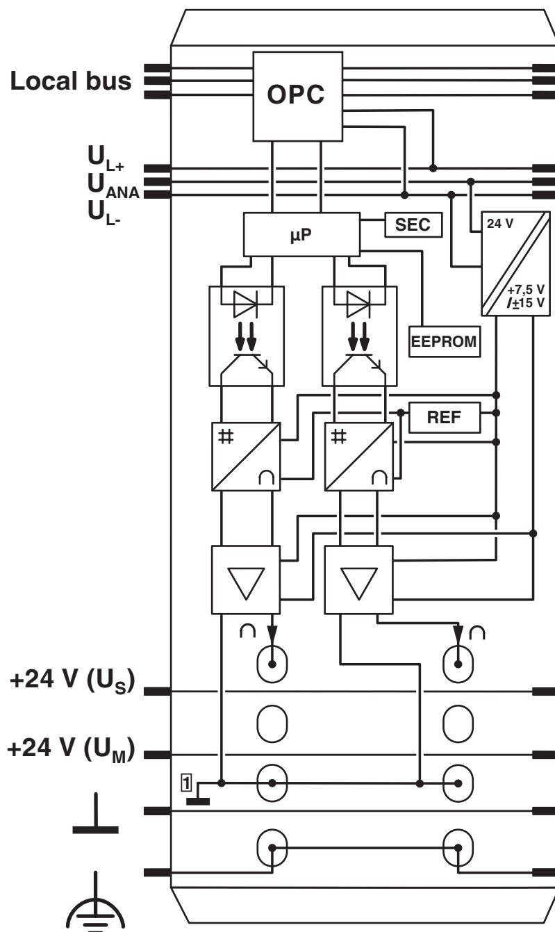
Block diagram
