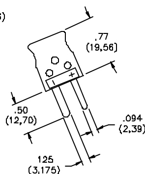
THERMO COUPLE EXTENSION WIRE WIRE LENGTH: 118 INCHES (3 METERS)
