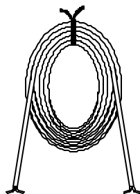
THERMO COUPLE EXTENSION WIRE WIRE LENGTH: 118 INCHES (3 METERS)
