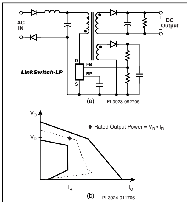
Figure 1. Typical Application – not a Simplified Circuit (a) and Output Characteristic Envelope (b).
