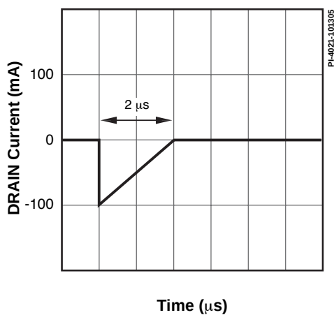
Figure 10. Peak Negative Pulsed DRAIN Current Waveform.
