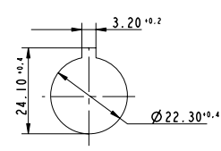
Panel cut-out to IEC 60947-5-1
