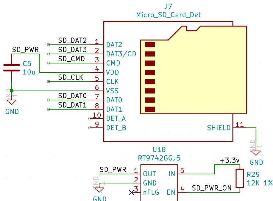
Figure 3. CM4Lite SD card interface.
