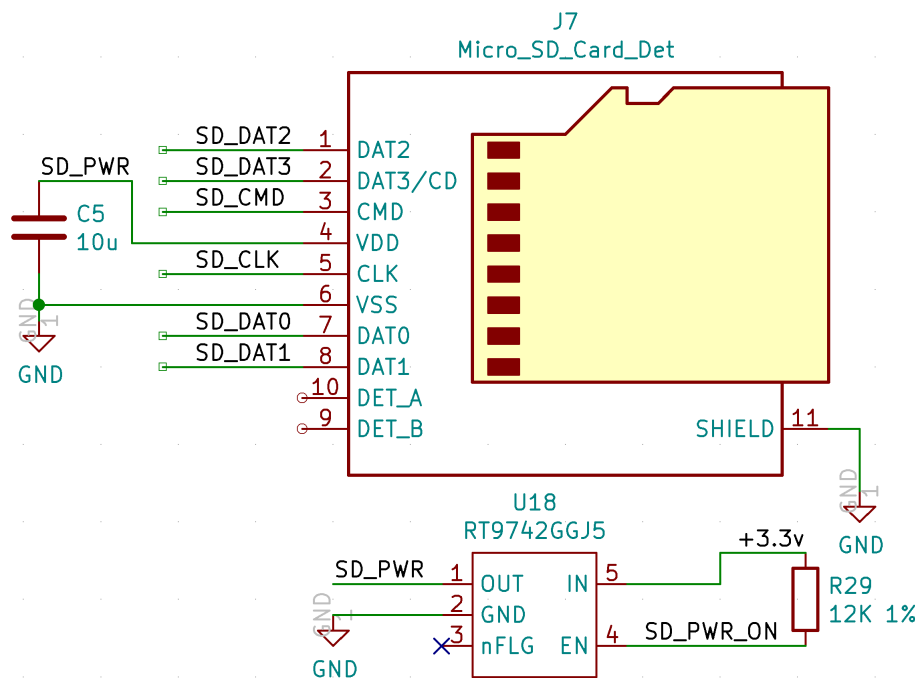
Figure 3. CM4Lite SD card interface.
