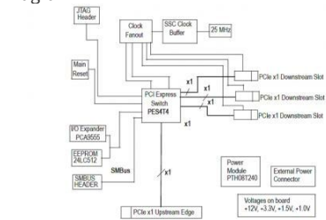
89KTPES3T3QFN Eval Board Functional Diagram
