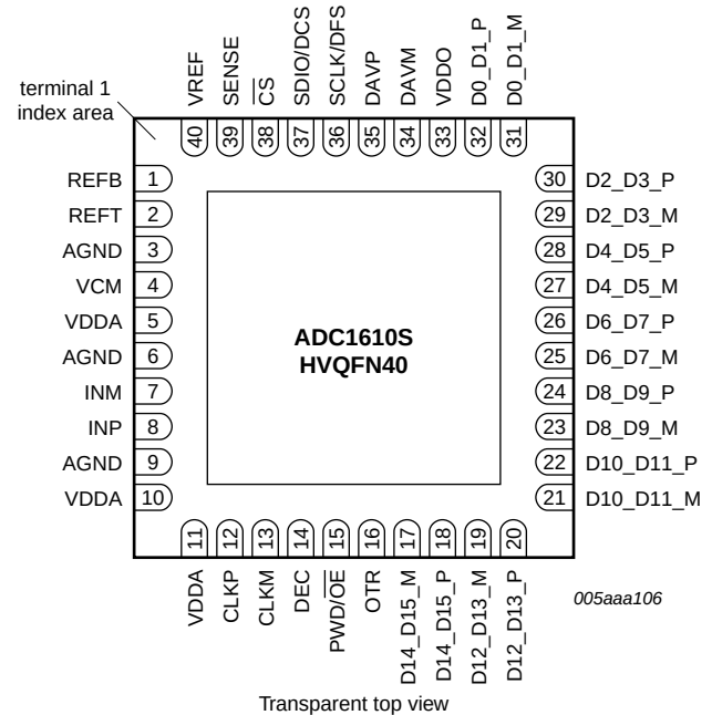
Fig 3. Pin configuration with LVDS DDR digital outputs selected
