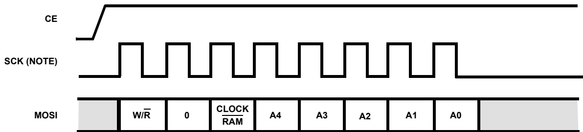
FIGURE 9. ADDRESS/CONTROL BYTE-TRANSFER WAVEFORMS
