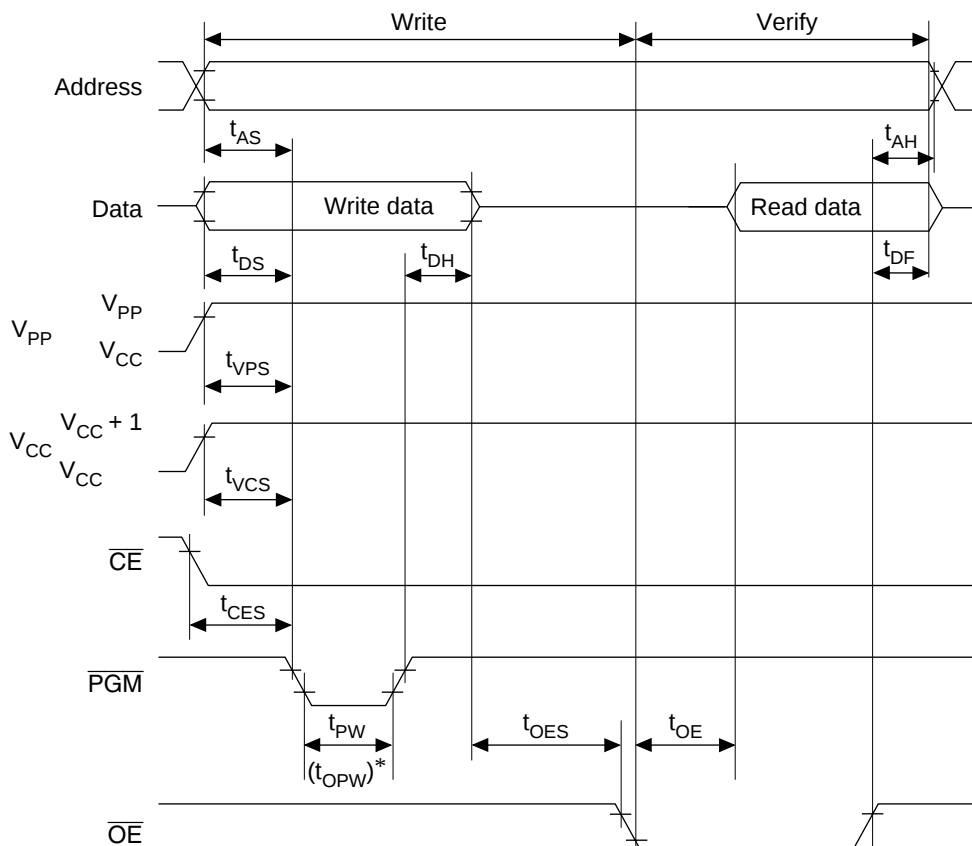
Figure 21.7 Write/Verify Timing
