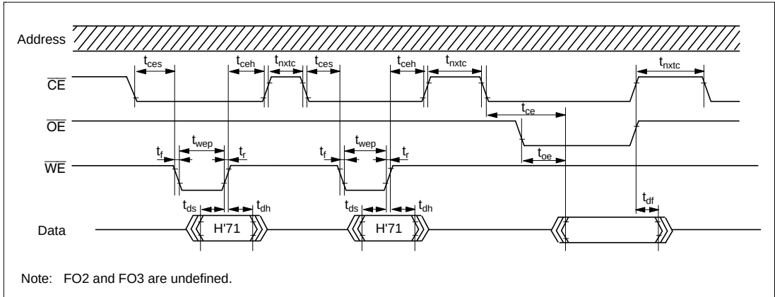
Figure 21.22 Status Read Mode Timing Waveforms
