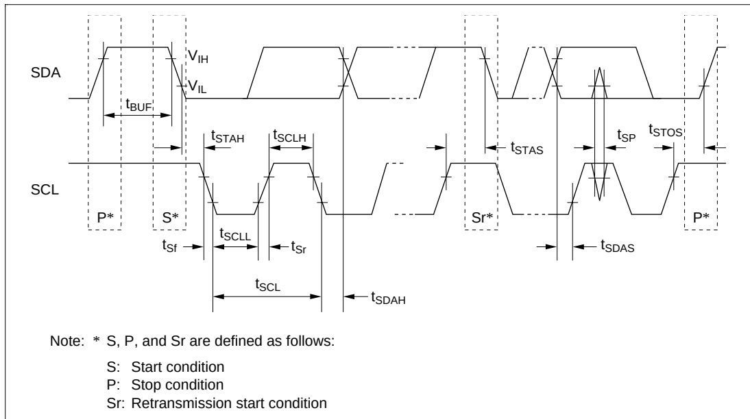
Figure 23.24 I 2 C Interface Input/Output Timing
