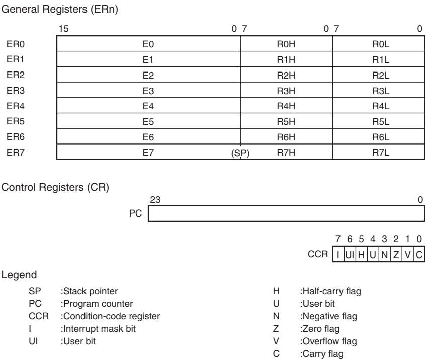
Figure 2.2 CPU Registers
