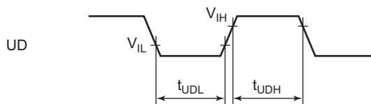
Figure 16.7 UD Pin Minimum Transition Width Timing
