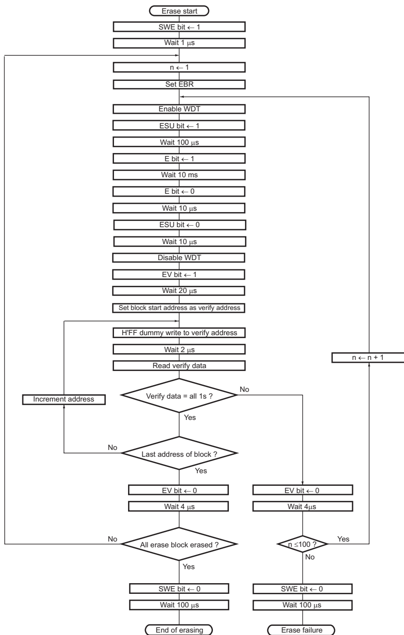
Figure 6.11 Erase/Eraser-Verify Flowchart
