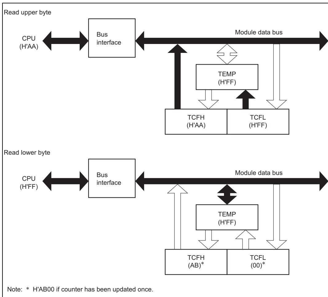
Figure 9.5 Read Access to TCF (TCF → CPU)
