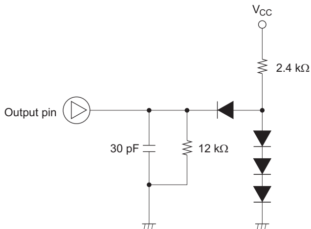
Figure 16.8 Output Load Condition
