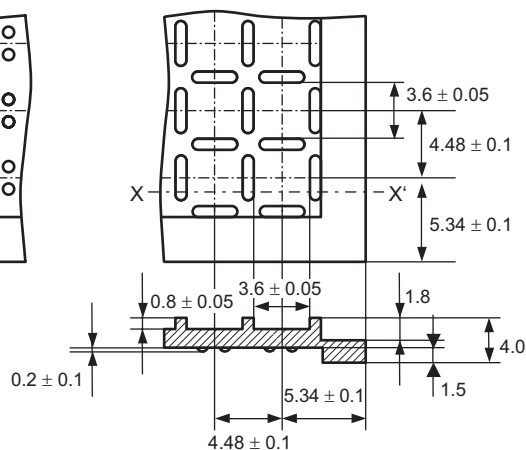
Figure I.3 Specifications of Chip Tray for the HCD64338024S, HCD64338023S, HCD64338022S, HCD64338021S, and HCD64338020S
