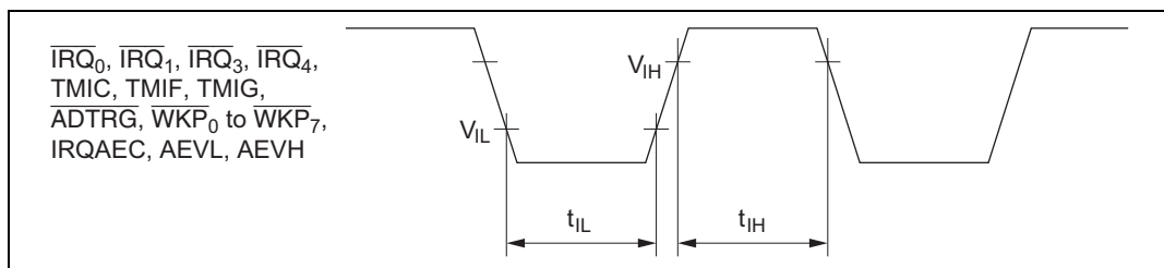
Figure 16.4 Input Timing
