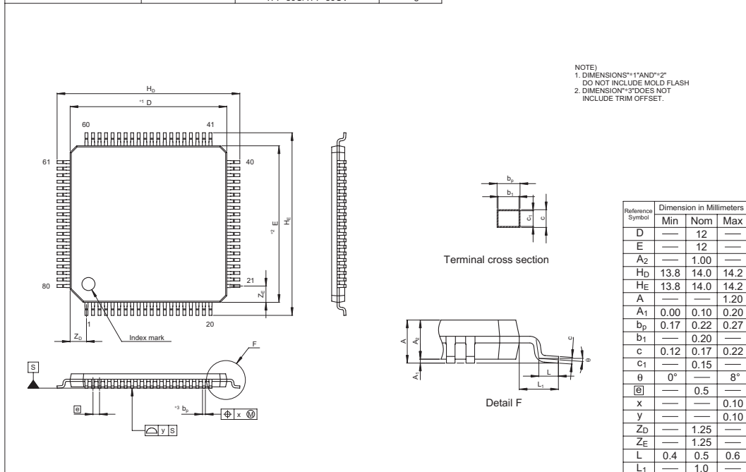
Figure F.3 TFP-80C Package Dimensions
