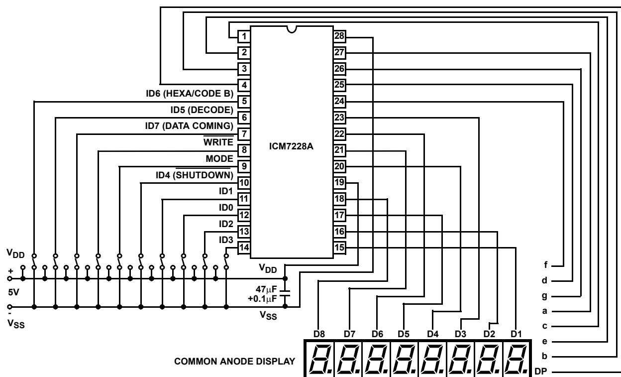
FIGURE 18. FUNCTIONAL TEST CIRCUIT #1
