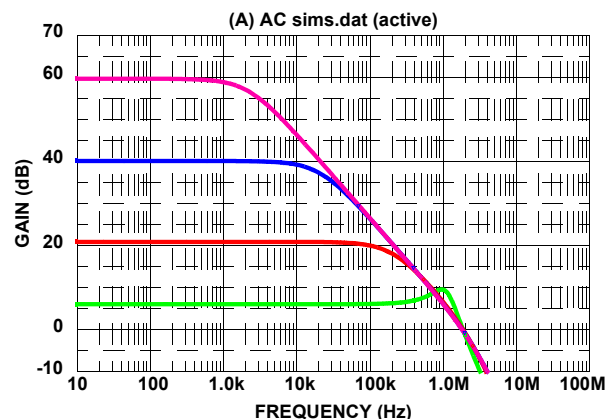
FIGURE 26. SIMULATED CLOSED LOOP GAIN vs FREQUENCY
