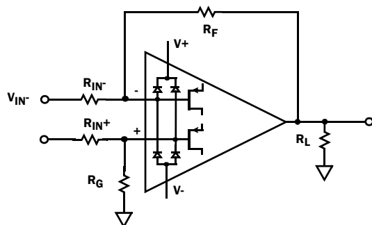
FIGURE 19. INPUT ESD DIODE CURRENT LIMITING
