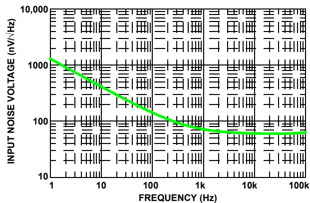
FIGURE 24. SIMULATED INPUT NOISE VOLTAGE
