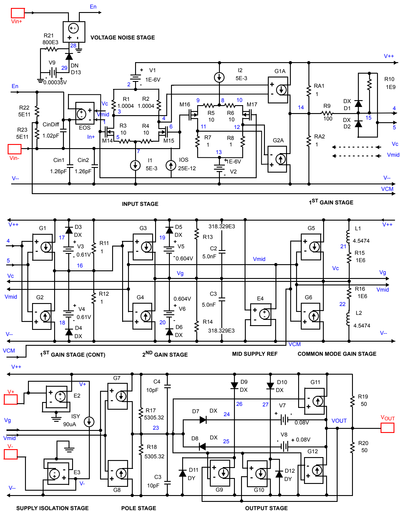
FIGURE 21. SPICE SCHEMATIC
