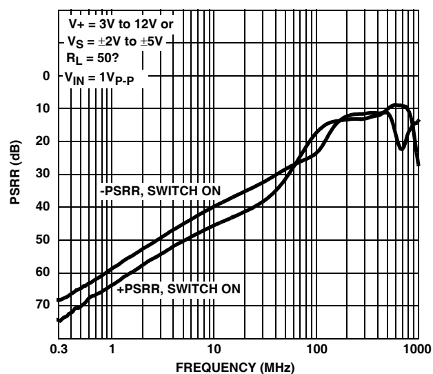
FIGURE 21. \pm PSRR vs FREQUENCY
