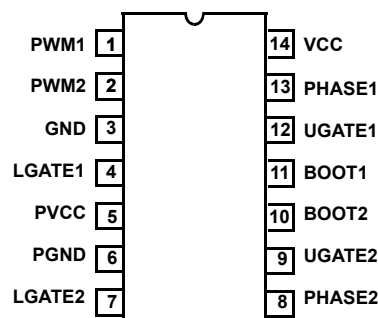
ISL6614ACB, ISL6614ACBZ, ISL6614ACBZA, ISL6614AIB, ISL6614AIBZ 14 LD SOIC TOP VIEW
