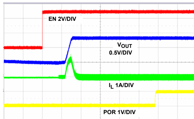
FIGURE 20. SOFT-START WITH PRE-BIASED 1V, 500μs/DIV
