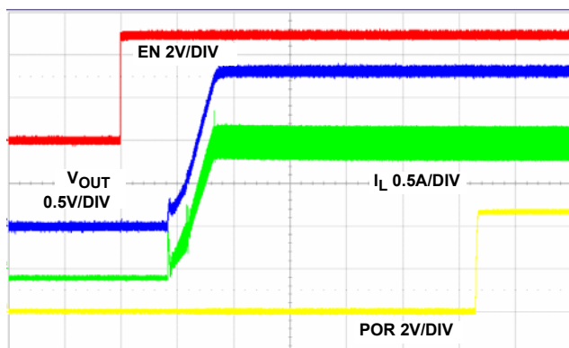
FIGURE 21. SOFT-START AT FULL LOAD, 500μs/DIV
