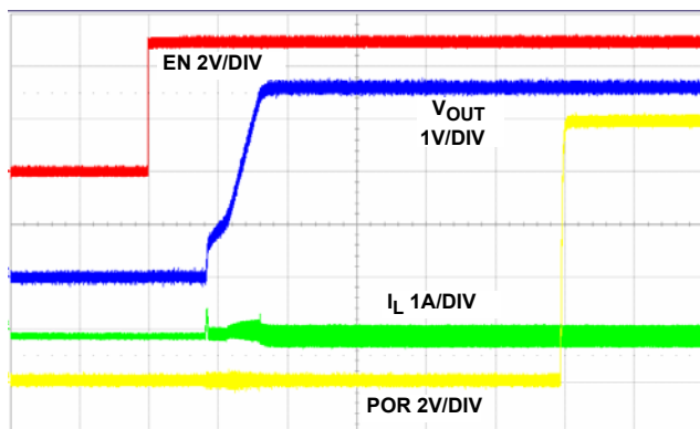
FIGURE 19. SOFT-START AT NO LOAD, 500μs/DIV
