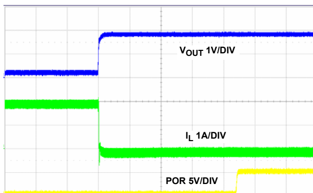
FIGURE 23. OUTPUT SHORT CIRCUIT RECOVERY, 500μs/DIV
