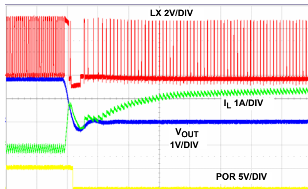
FIGURE 22. OUTPUT SHORT CIRCUIT, 10.0μs/DIV
