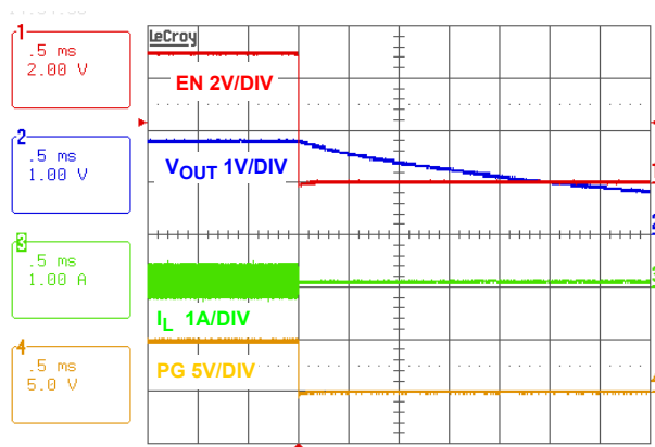
FIGURE 38. SOFT-DISCHARGE SHUTDOWN
