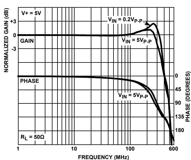
FIGURE 13. FREQUENCY RESPONSE
