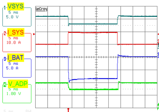
FIGURE 16. BOOST MODE, OUTPUT VOLTAGE LOOP TO INPUT VOLTAGE LOOP TRANSITION. V_{ADP} = 5.004V , MAXSYSTEMVOLTAGE = 12.576V , V_{BAT} = 11V , VINDAC = 4.437V , SYSTEM LOAD 0A TO 10A STEP , CHARGECURRENT = 0A
