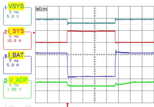
FIGURE 17. BOOST MODE, CHARGING CURRENT LOOP TO INPUT VOLTAGE LOOP TRANSITION. V_{ADP} = 5.004V , MAXSYSTEMVOLTAGE = 12.576V , V_{BAT} = 11V , VINDAC = 4.437V , SYSTEM LOAD 0A TO 10A STEP , CHARGECURRENT = 0.5A
