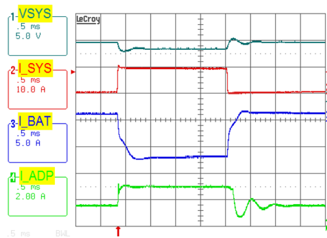
FIGURE 13. BUCK-BOOST MODE, CHARGING CURRENT LOOP TO ADAPTER CURRENT LOOP TRANSITION. V_{ADP} = 12V , MAXSYSTEMVOLTAGE = 12.576V , V_{BAT} = 11V , SYSTEM LOAD 1A TO 10A STEP, ADAPTERCURRENTLIMIT = 3A , CHARGECURRENT = 1A
