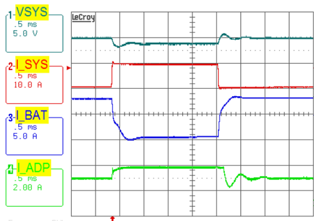
FIGURE 15. BUCK MODE, CHARGING CURRENT LOOP TO ADAPTER CURRENT LOOP TRANSITION. V_{ADP} = 20V , MAXSYSTEMVOLTAGE = 12.576V , V_{BAT} = 11V , SYSTEM LOAD 2A TO 10A STEP , ADAPTERCURRENTLIMIT = 3A , CHARGECURRENT = 3A
