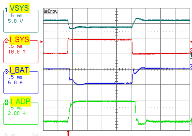
FIGURE 14. BUCK MODE, OUTPUT VOLTAGE LOOP TO ADAPTER CURRENT LOOP TRANSITION. V_{ADP} = 20V , MAXSYSTEMVOLTAGE = 12.576V , V_{BAT} = 11V , SYSTEM LOAD 2A TO 10A STEP , ADAPTERCURRENTLIMIT = 3A , CHARGECURRENT = 0A
