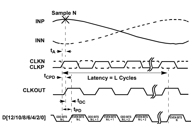
Figure 4. DDR
