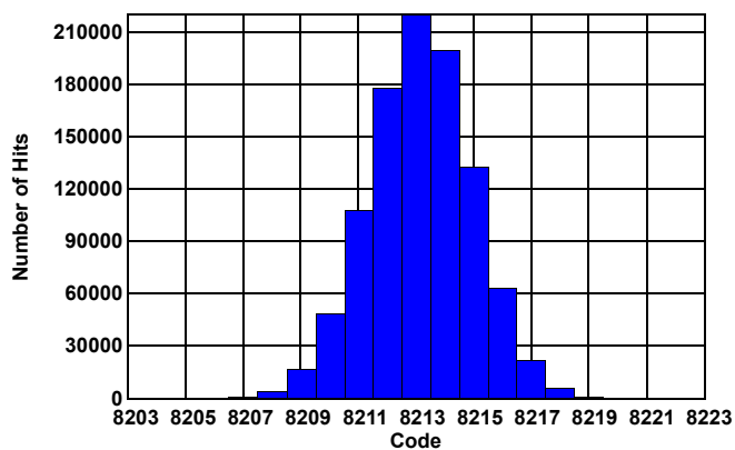
Figure 16. Noise Histogram
