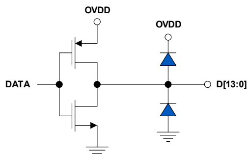
Figure 49. CMOS Outputs
