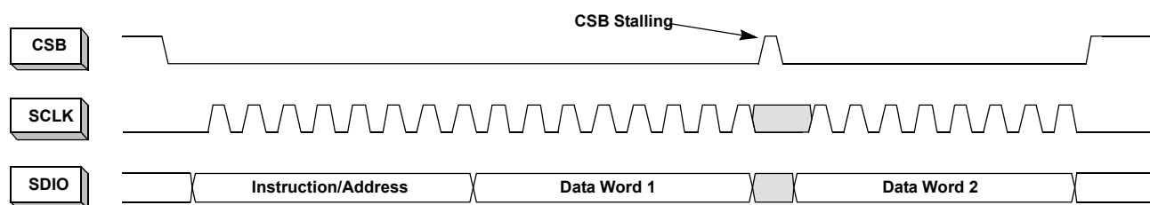
Figure 40. 2-Byte Transfer
