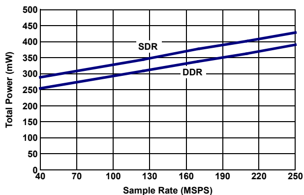
Figure 12. Power vs f_{SAMPLE} in 3mA LVDS Mode
