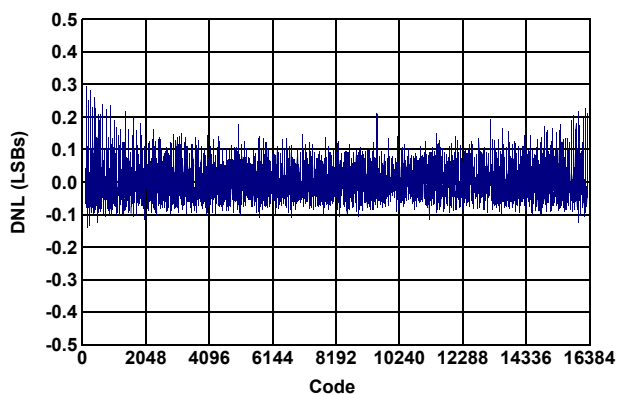
Figure 13. Differential Nonlinearity
