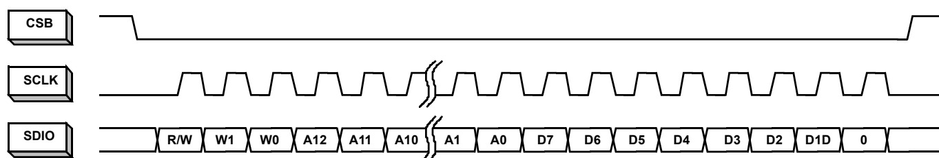
Figure 36. MSB-First Addressing
