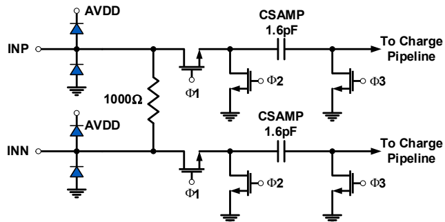
Figure 44. Analog Inputs
