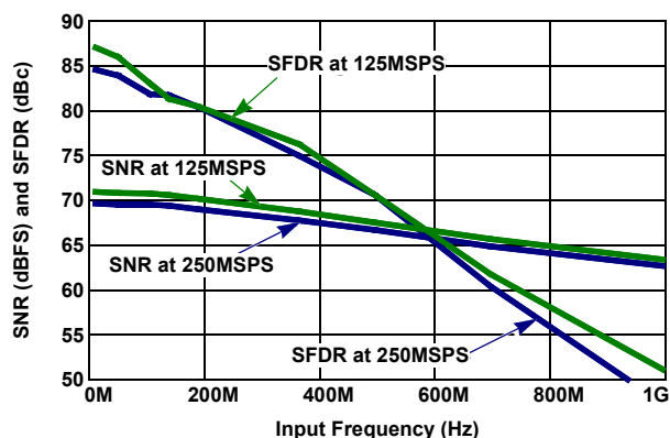
Figure 6. SNR and SFDR vs f_{IN}
