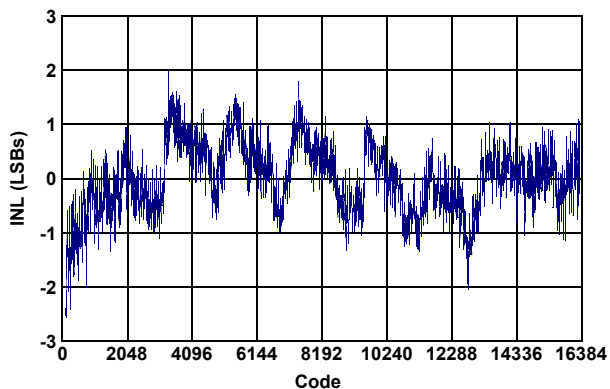
Figure 14. Integral Nonlinearity
