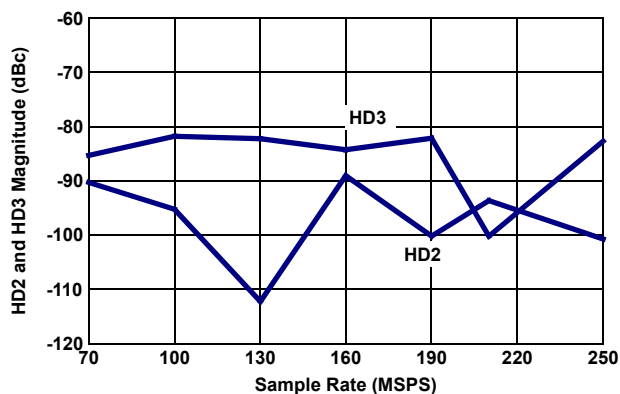
Figure 11. HD2 and HD3 vs f_{SAMPLE}
