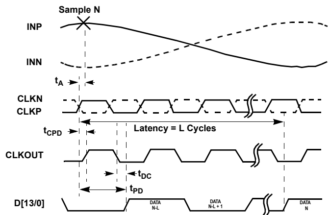
Figure 5. SDR
