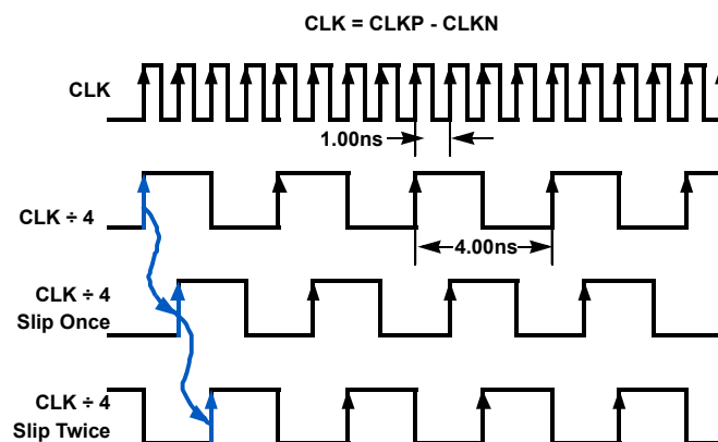
Figure 42. Phase Slip: CLK ÷ 4 Mode, f_{CLK} = 1000\text{MHz}
