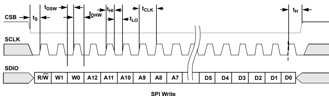
Figure 38. Write Timing
