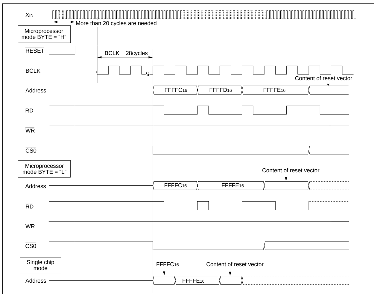
Figure 1.5.2. Reset sequence
