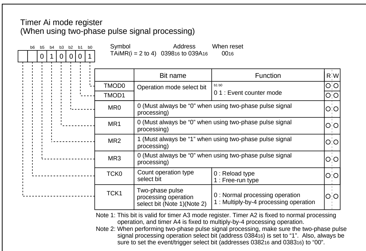
Figure 1.15.9. Timer Ai mode register in event counter mode
