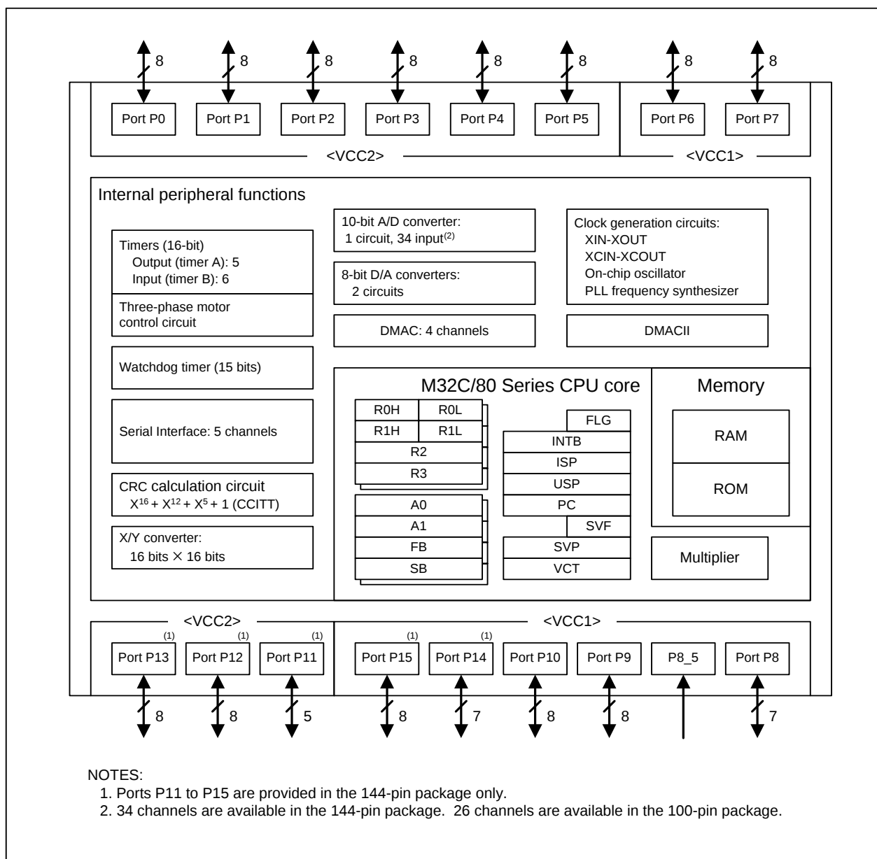
Figure 1.2 Block Diagram
