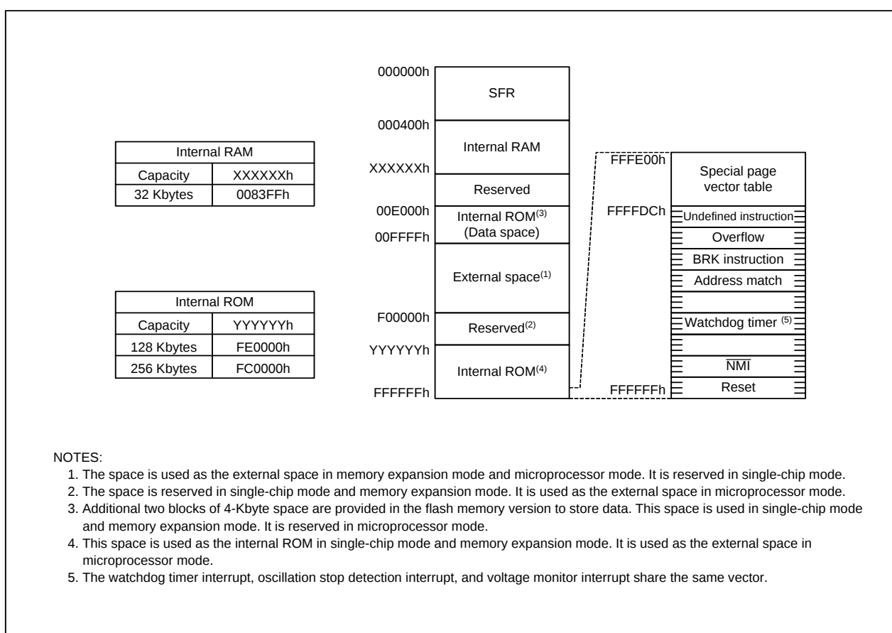
Figure 3.1 Memory Map
