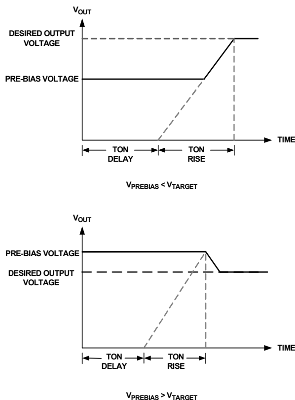
FIGURE 7. OUTPUT RESPONSES TO PREBIAS VOLTAGES
