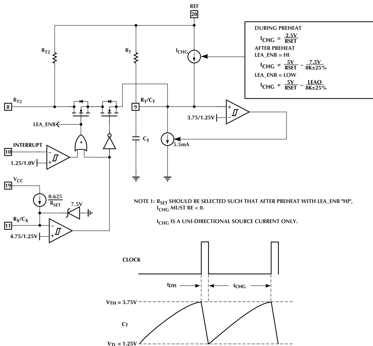
Figure 8. Oscillator Block Diagram and Timing
