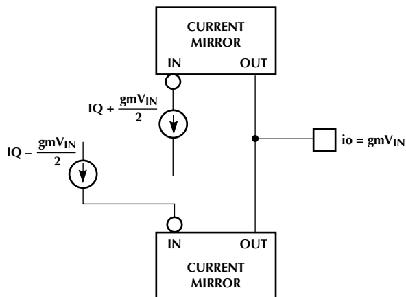
Figure 6. Output Configuration
